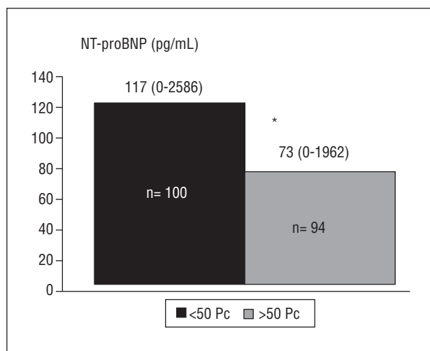
Fig. 2. Plasma concentration of NT-proBNP in the upper and lower 50th percentile of AVPD.
