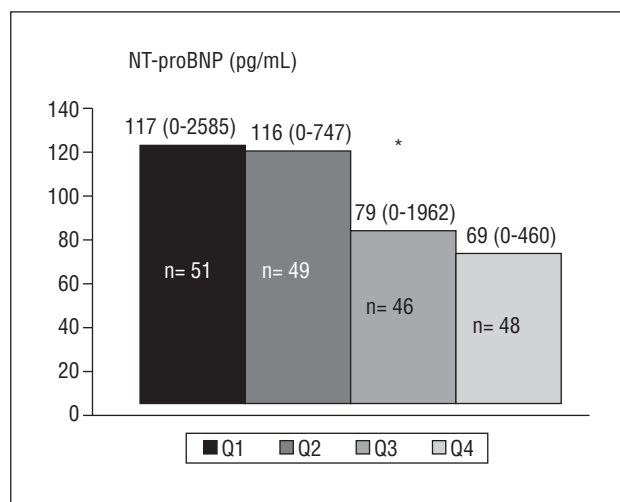
Fig. 1. Plasma concentration of NT-proBNP in each group according to quartile of AVPD.
