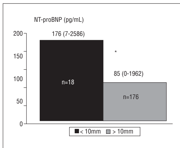
Fig. 3. Plasma concentration of NT-proBNP in patients with AVPD above and below the cut-off value of 10 mm.
