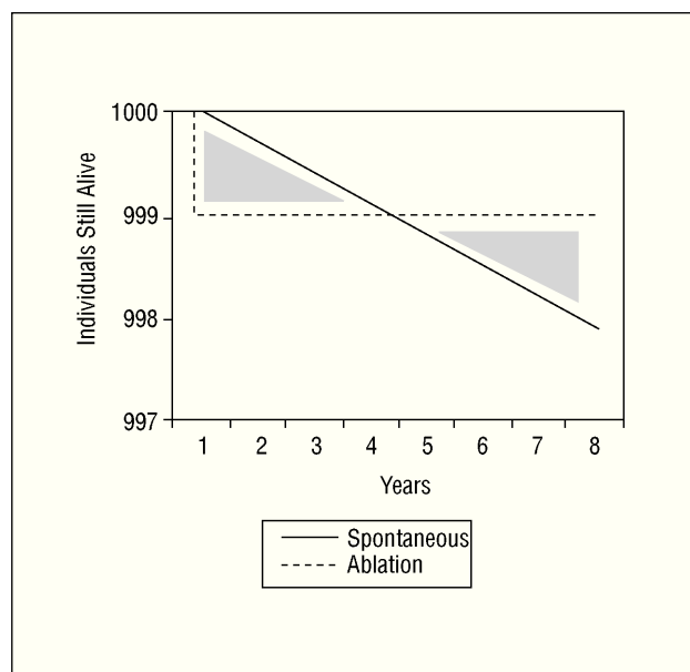
Fig. 4. Density of incidence of sudden death, plotted over time for an imaginary initial group of 1000 patients.
