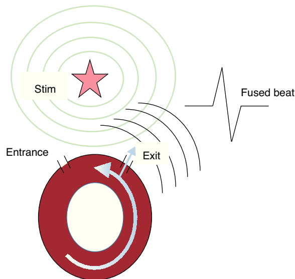
Figure 13. Schematic representation of a fused beat. Stim, stimulus.
