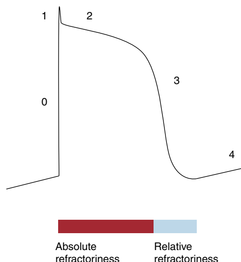
Figure 2. Refractory periods, showing the absolute and relative refractory periods during the action potential.
