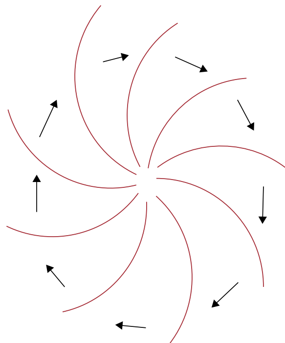
Figure 11. Schematic representation of a spiral wave.
