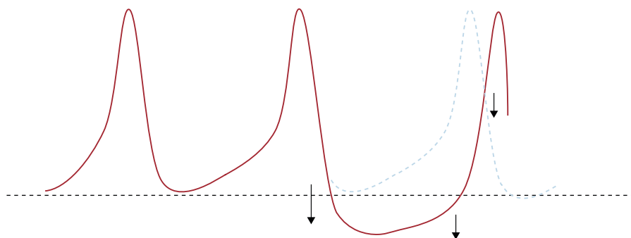
Figure 4. Parasympathetic effects on the action potential (reduction of the heart rate).
