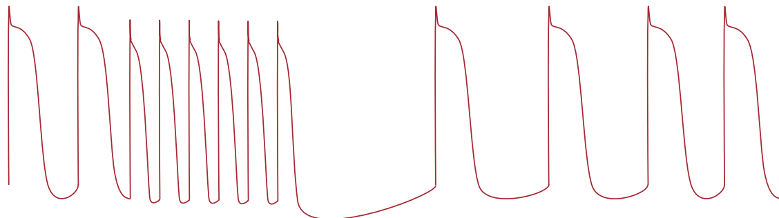
Figure 5. Overdrive suppression in a Purkinje fiber and postsuppression warm-up period.
