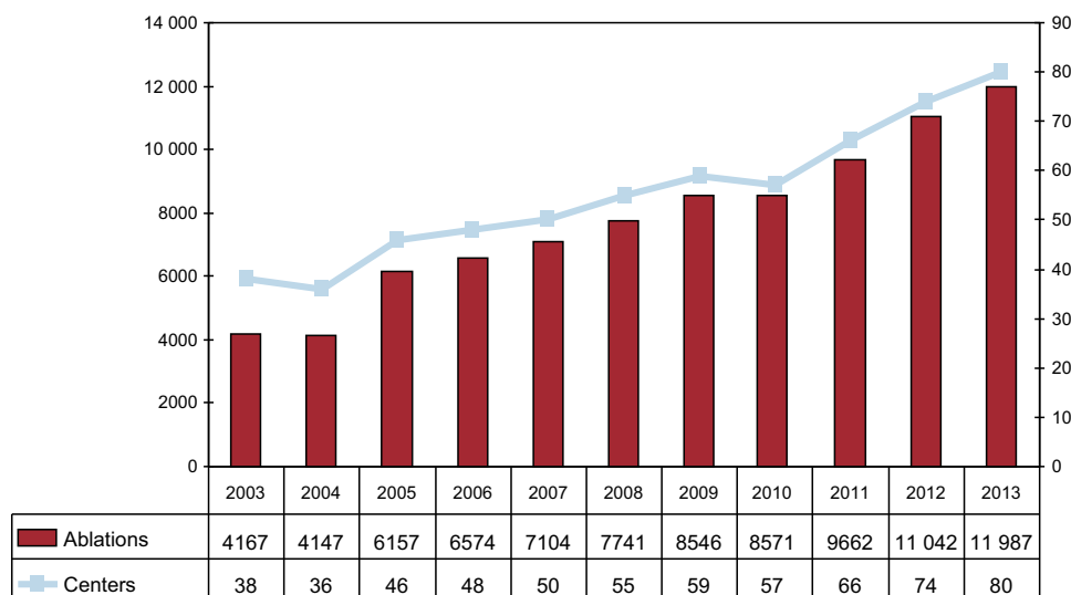
Figure 1. Data analyzed.
