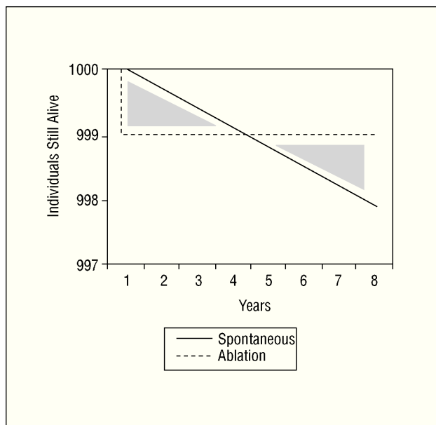
Fig. 4. Density of incidence of sudden death, plotted over time for an imaginary initial group of 1000 patients. Spontaneous indicates spontaneous clinical course of the patient group; ablation, clinical course of patients treated with catheter ablation who die on the day of the procedure (immediate mortality equivalent to sudden death) but then there are no more deaths, assuming 100% success rate and no recurrences (see text). The shaded triangles represent the difference in mortality in principle favorable to the conservative approach (lives gained). After the curves cross, ablation is favorable (lives lost). Ablation starts to be beneficial from the moment when the triangles have the same area, about 8 years after diagnosis.
